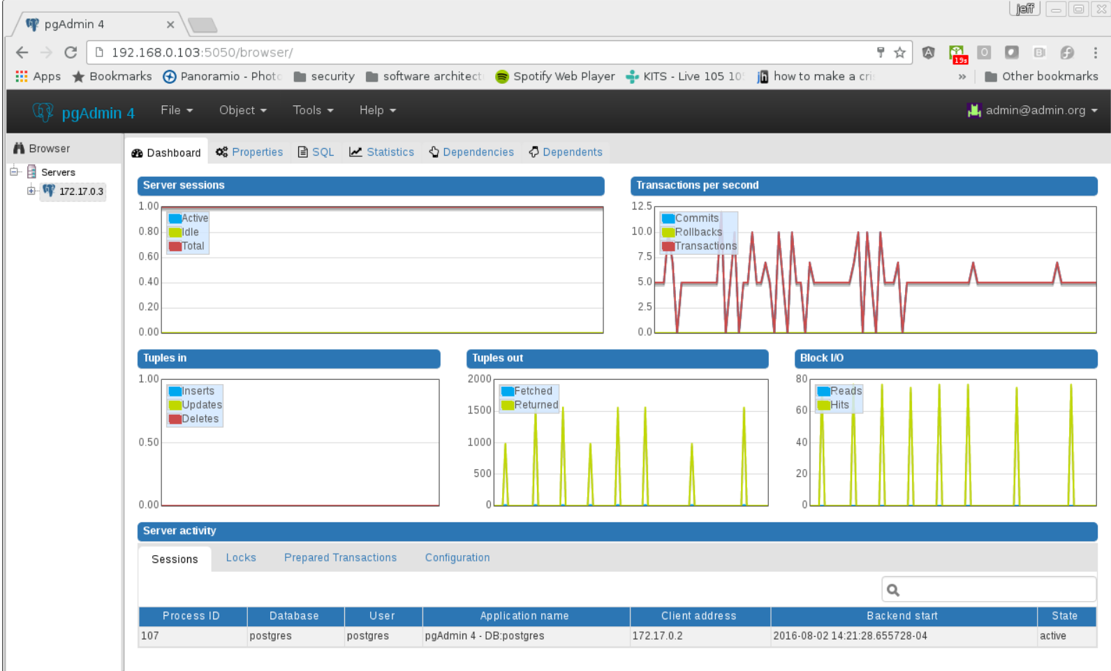
Figure 4: pgAdmin4
