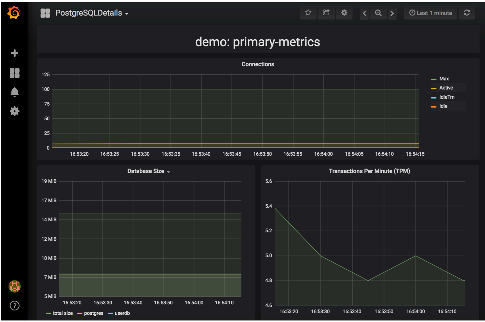
Figure 2: grafana
