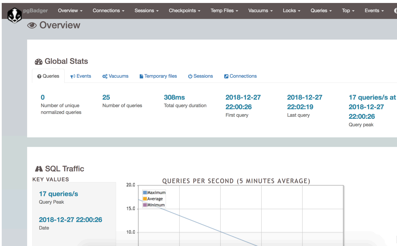
Figure 3: pgbadger
