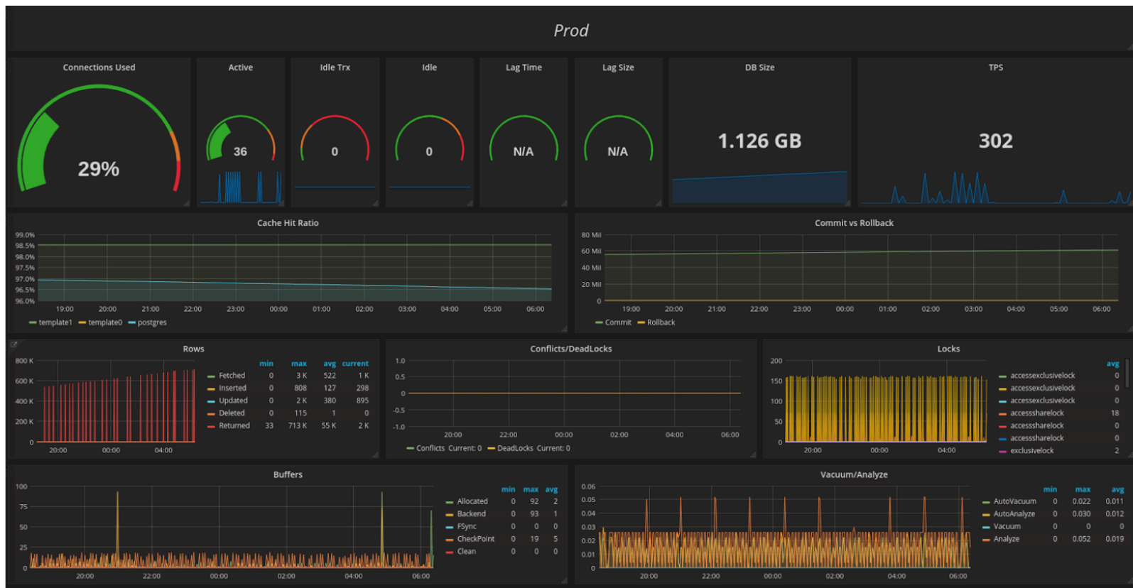
Figure 1: pgmonitor
