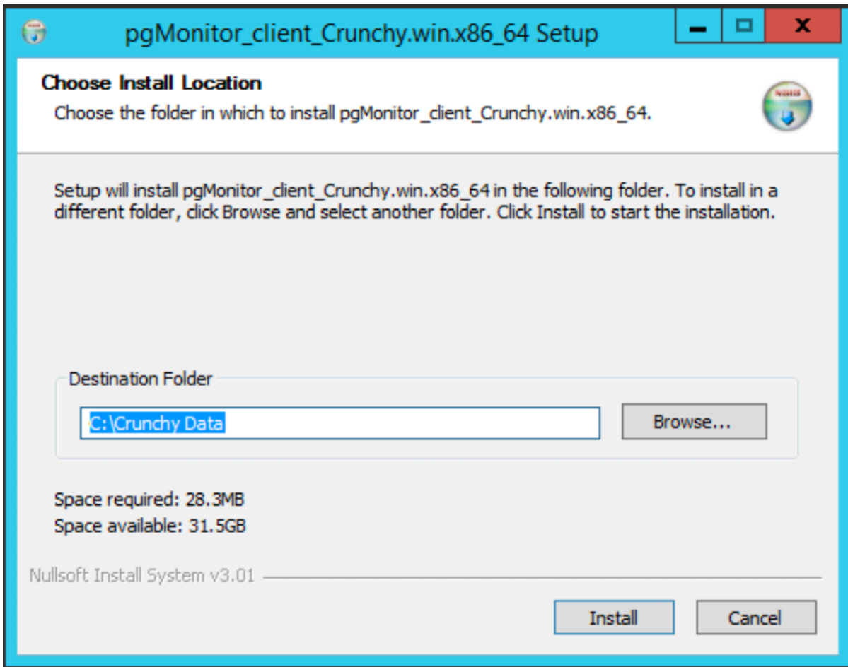
Figure 1: client installer 1
