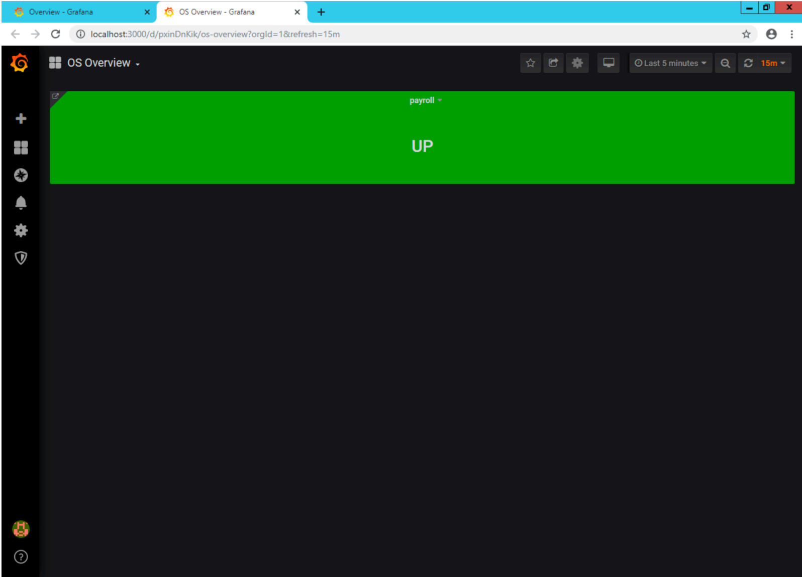
Figure 30: server_installer_17
