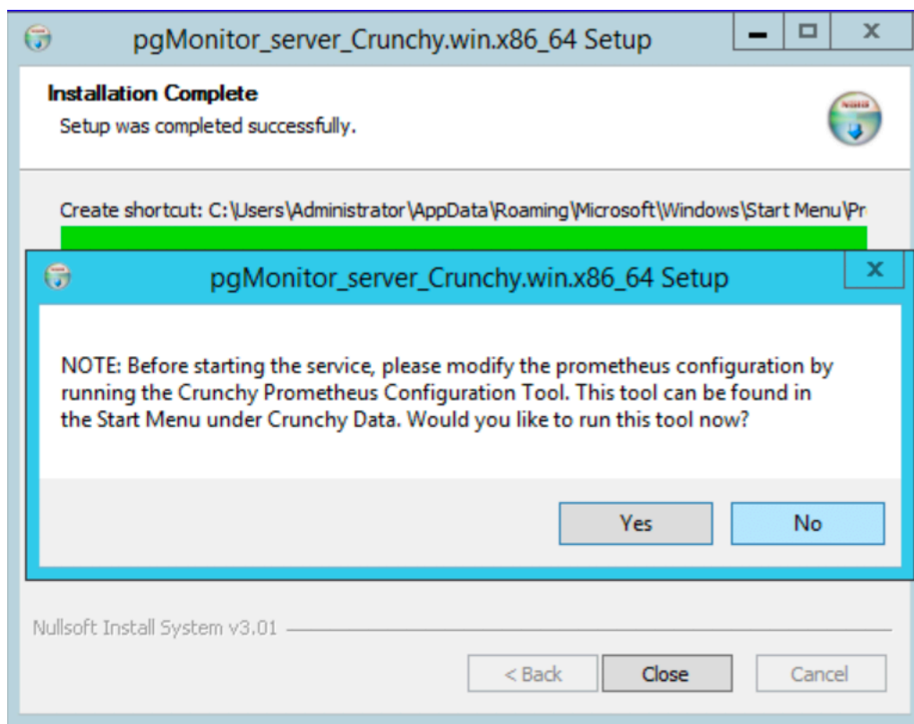
Figure 17: server_installer_4.png
