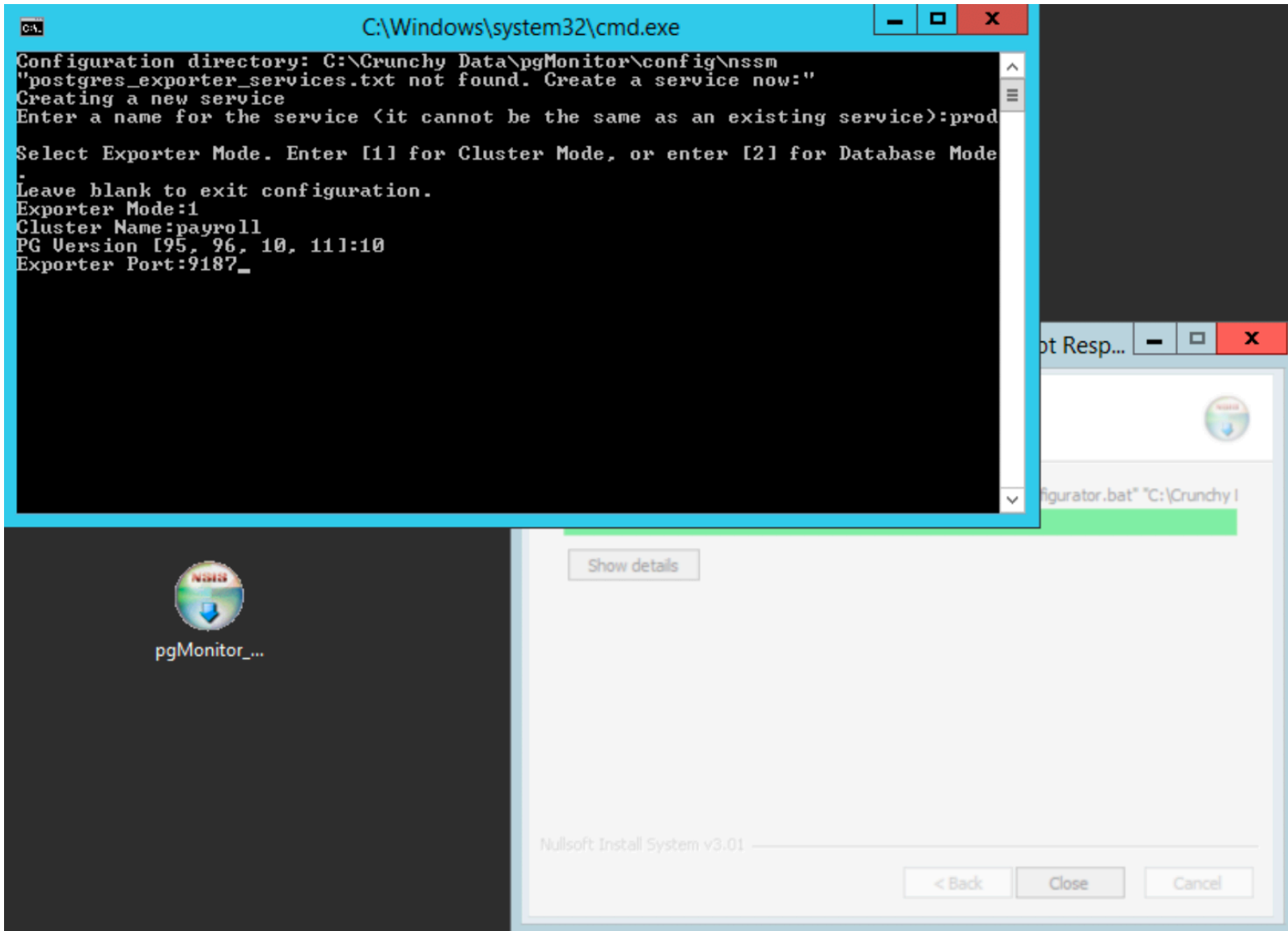
Figure 7: client installer 7
