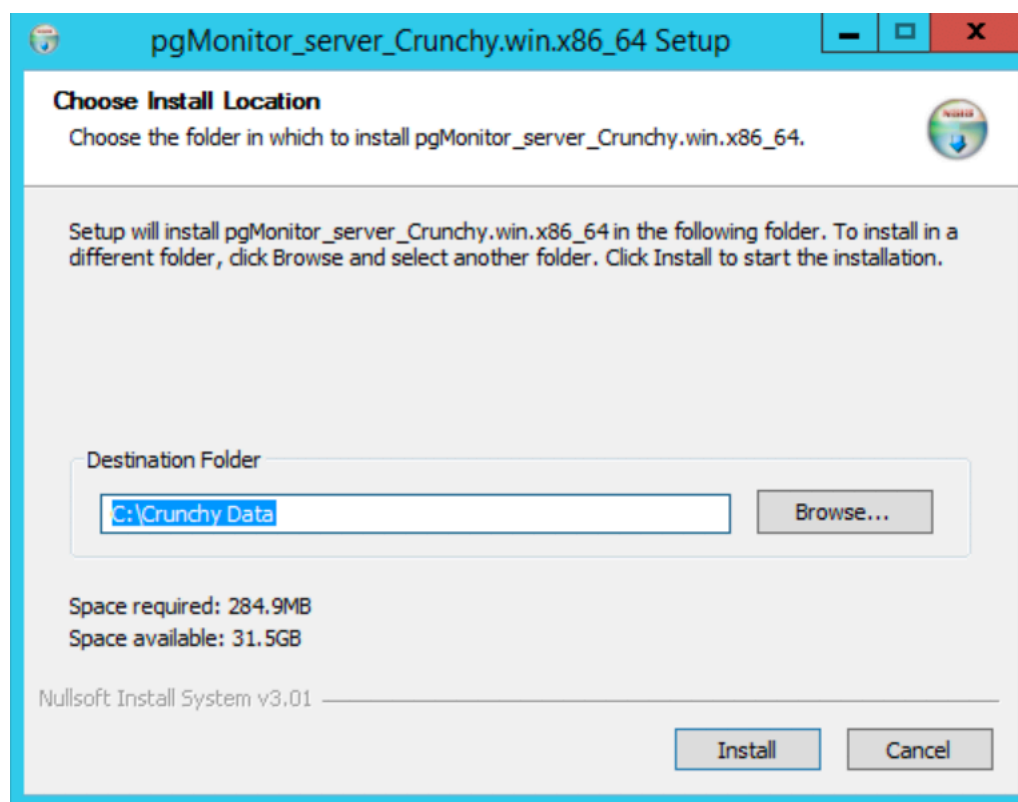
Figure 14: server_installer_1.png
