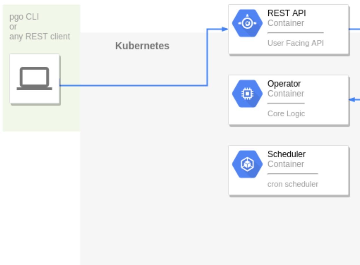
Figure 1: Architecture
