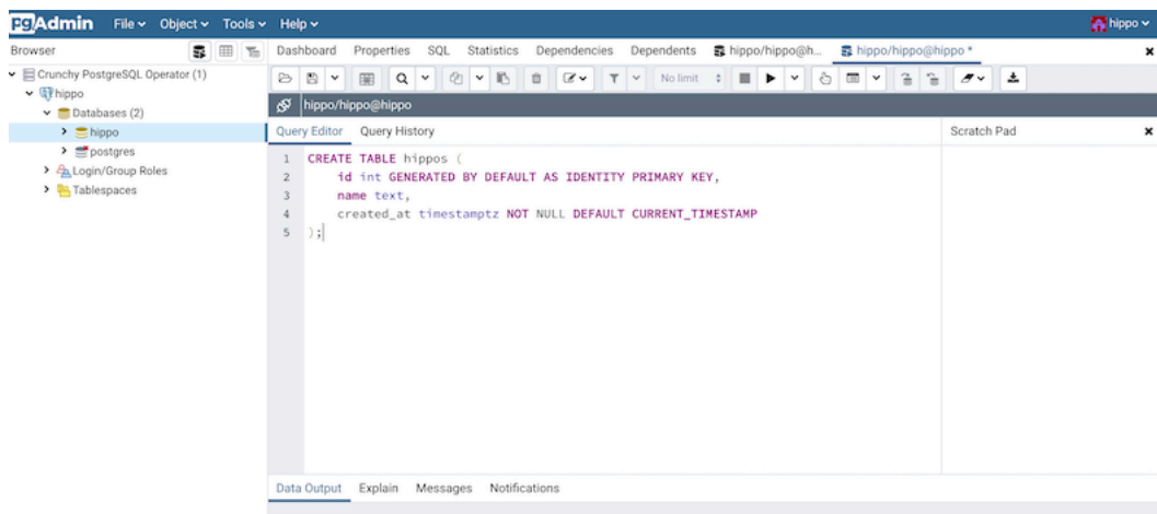
Figure 33: pgAdmin 4 Query
