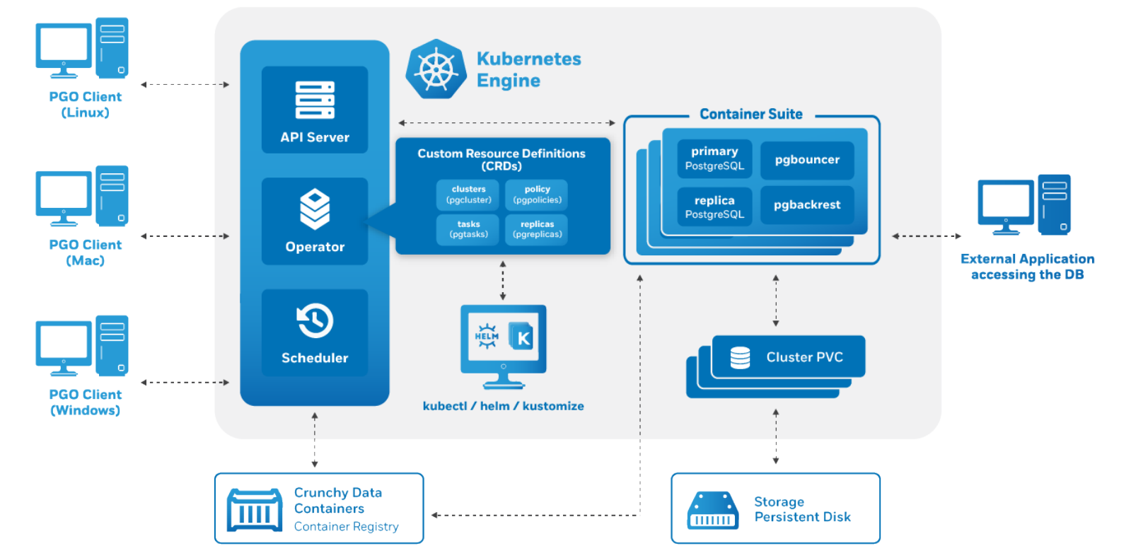
Figure 34: Operator Architecture with CRDs
