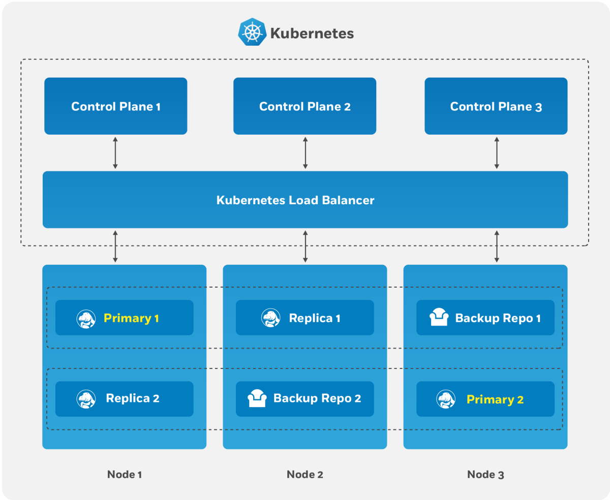
Figure 29: PostgreSQL Operator High-Availability Overview
