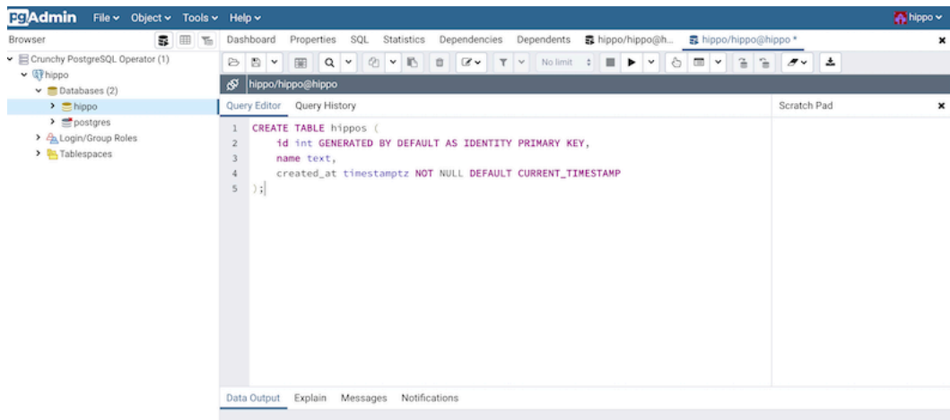
Figure 27: pgAdmin 4 Query
