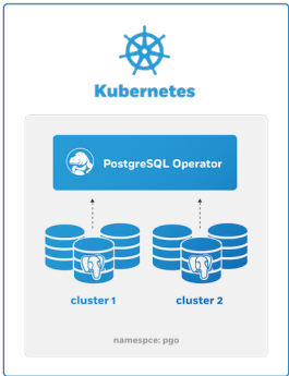
Figure 24: PostgreSQL Operator Own Namespace Deployment
