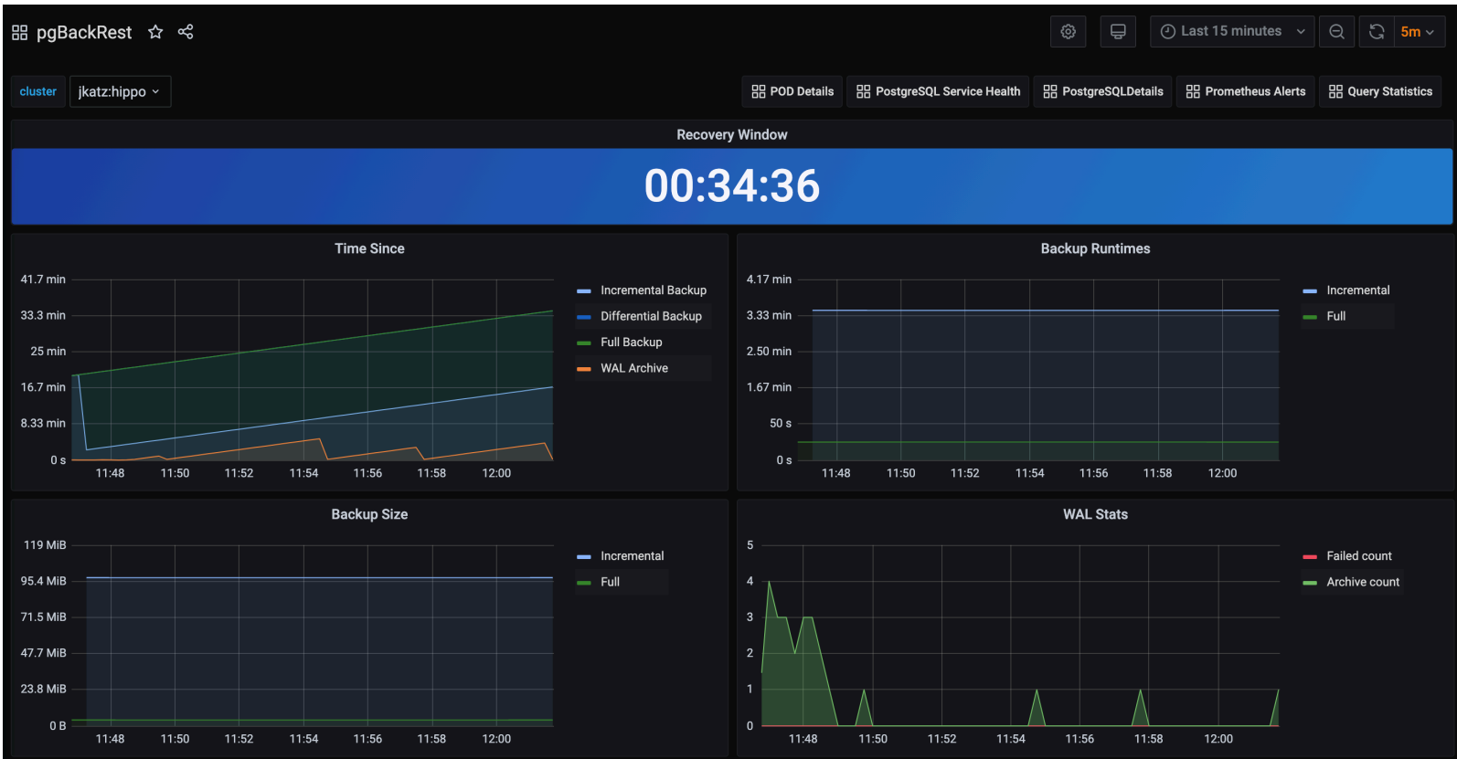
Figure 19: PostgreSQL Operator - Monitoring - Backup Health
