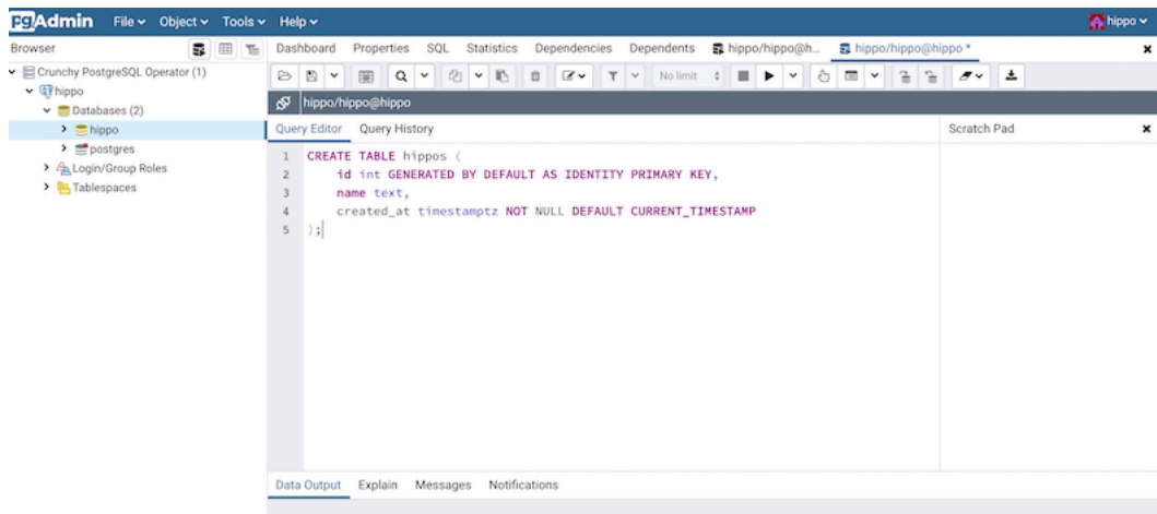
Figure 27: pgAdmin 4 Query
