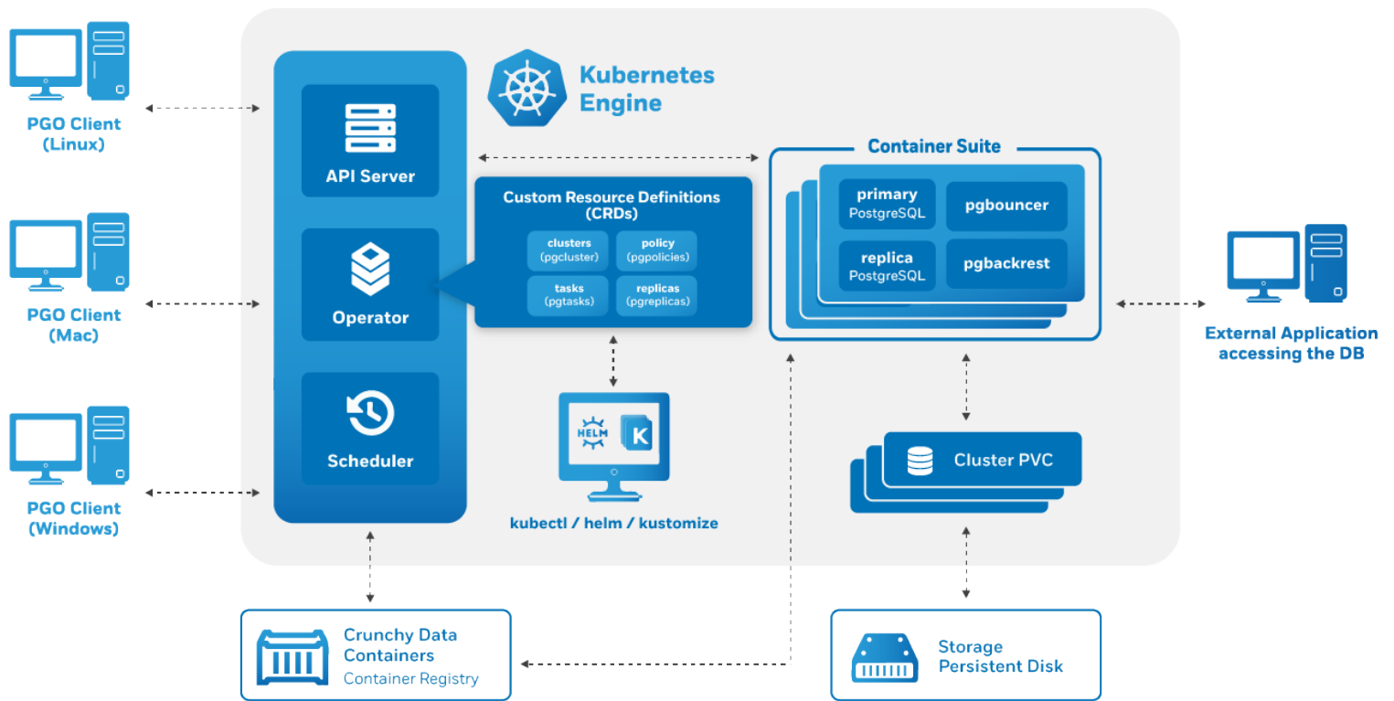
Figure 31: Architecture
