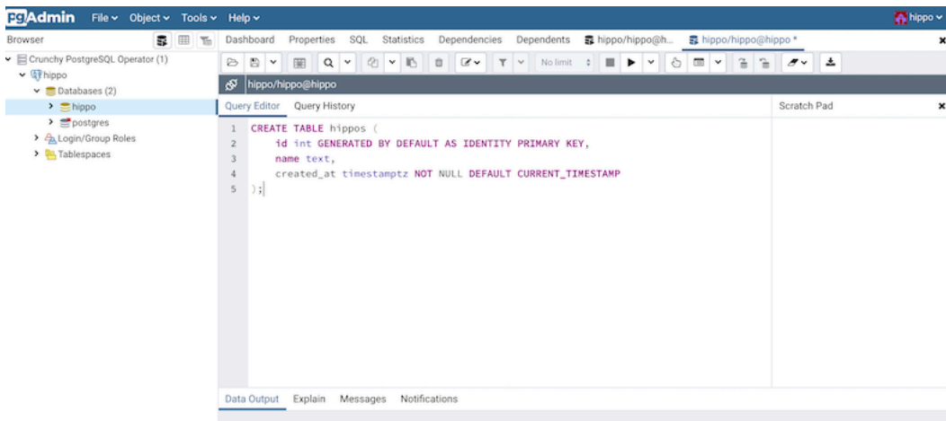
Figure 27: pgAdmin 4 Query
