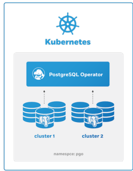
Figure 24: PostgreSQL Operator Own Namespace Deployment
