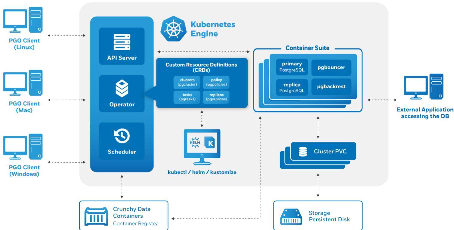
Figure 34: Operator Architecture with CRDs
