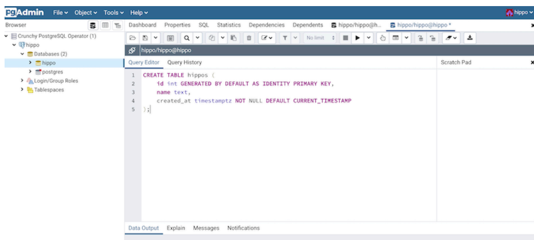
Figure 33: pgAdmin 4 Query
