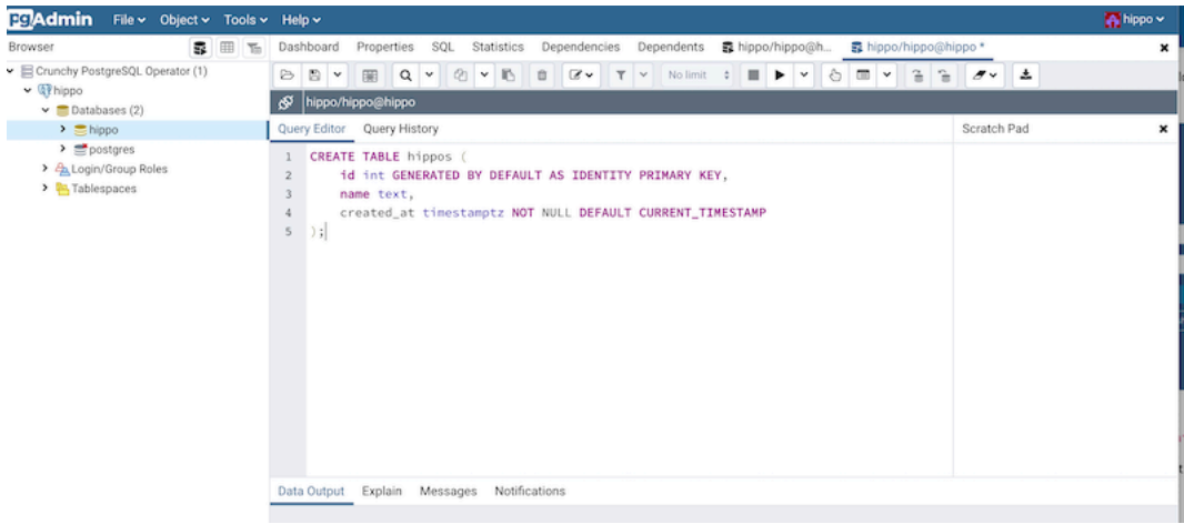
Figure 27: pgAdmin 4 Query
