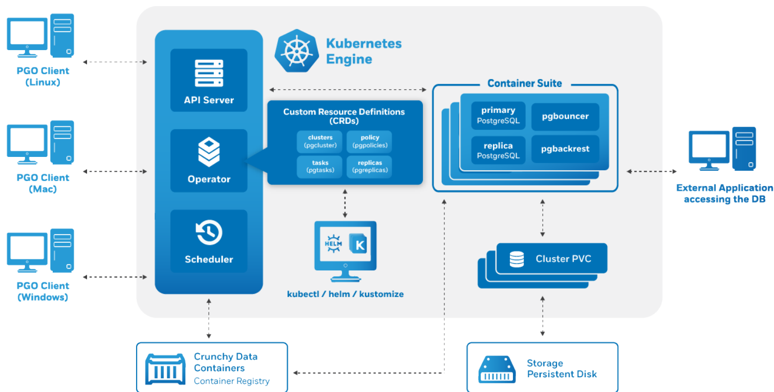
Figure 31: Architecture
