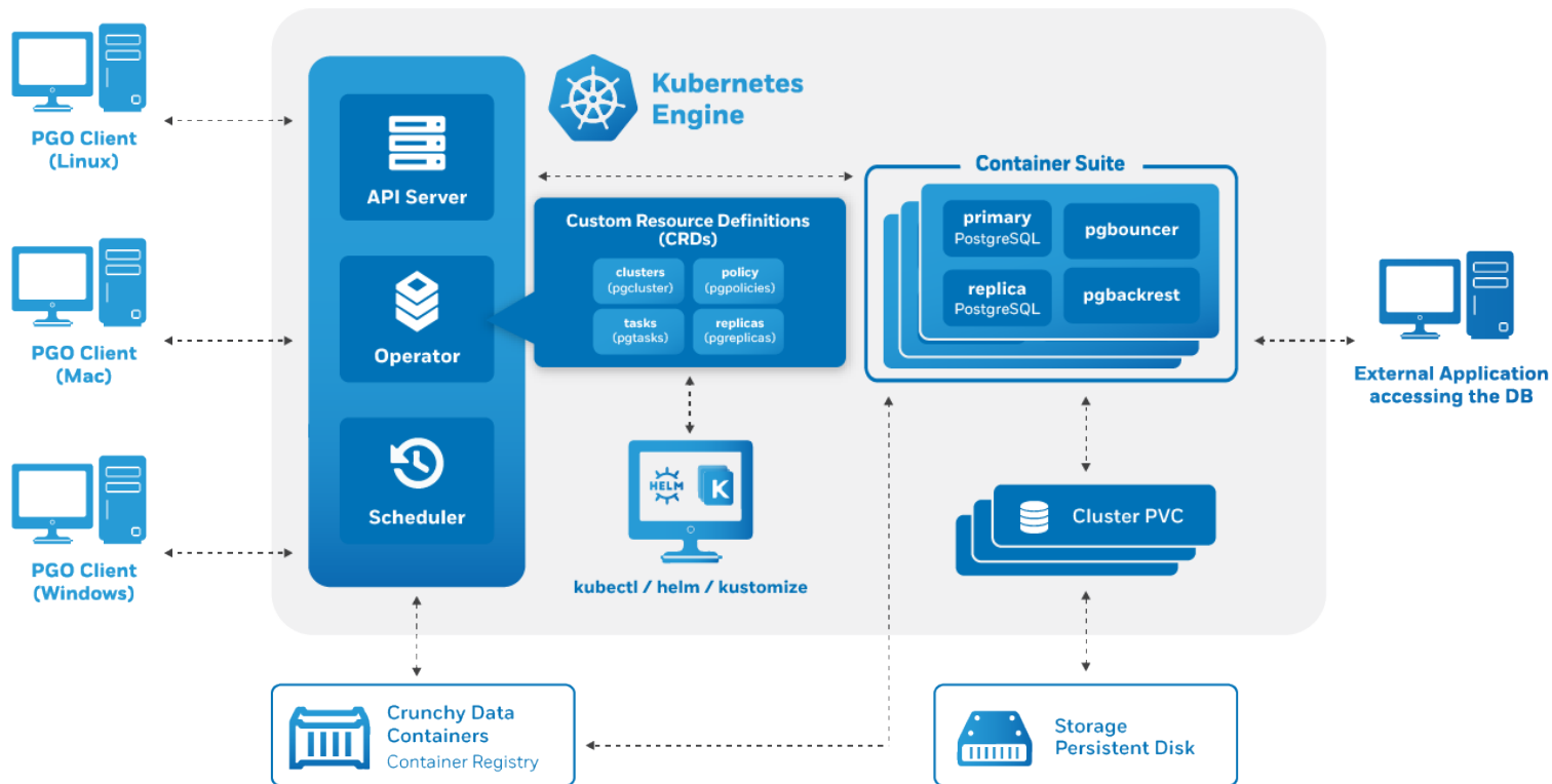
Figure 34: Operator Architecture with CRDs
