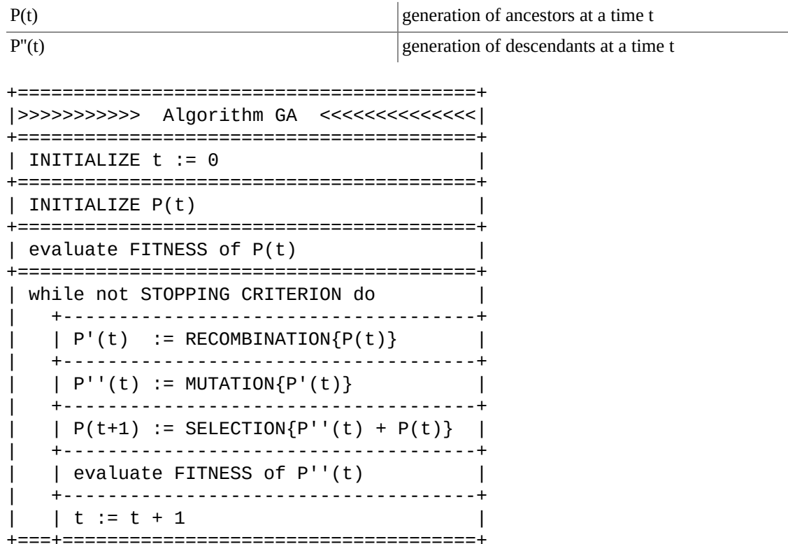
Figure 59.1. Structured Diagram of a Genetic Algorithm
