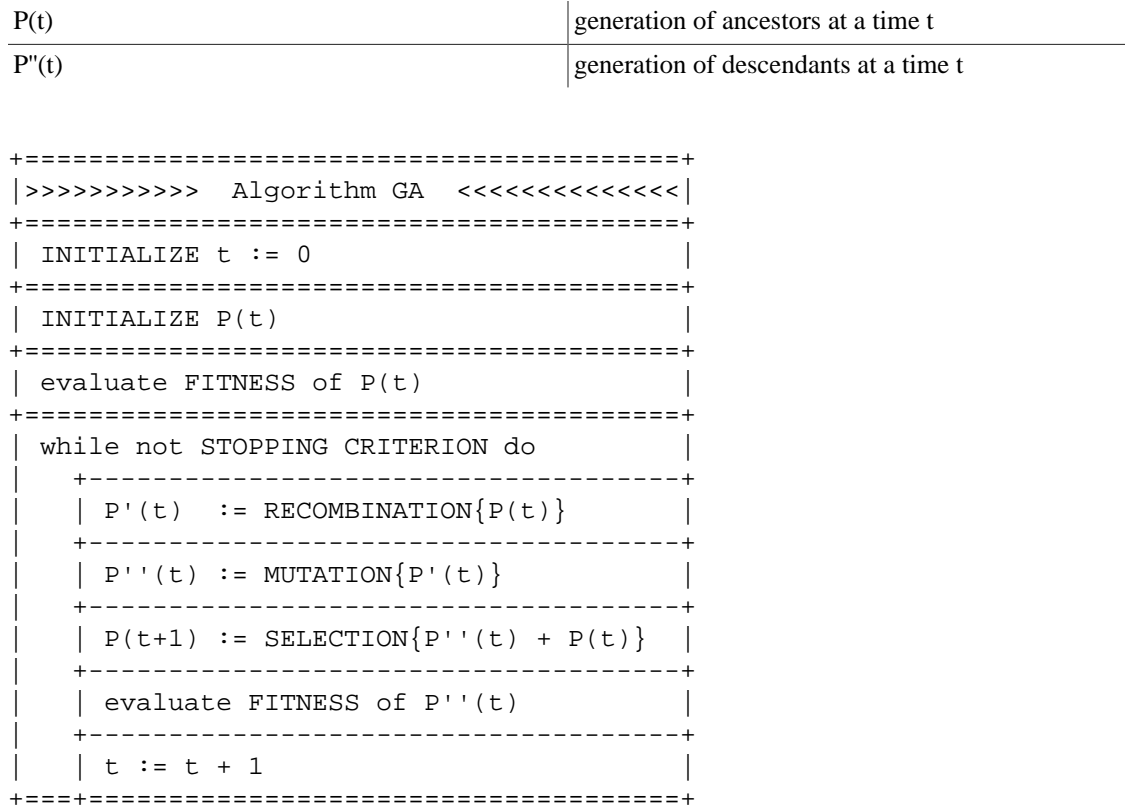
Figure 60.1. Structured Diagram of a Genetic Algorithm
