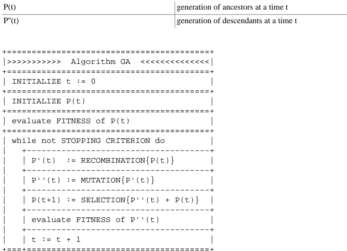
Figure 59.1. Structured Diagram of a Genetic Algorithm
