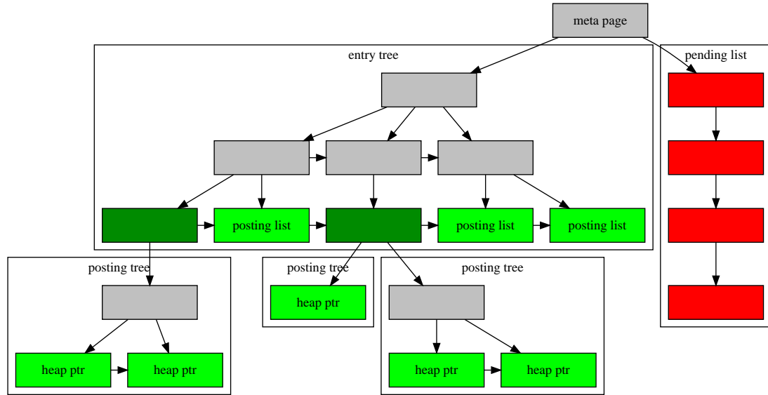
Figure 66.1. GIN Internals
