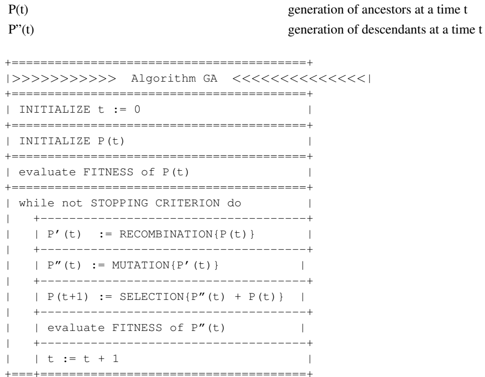
Figure 54-1. Structured Diagram of a Genetic Algorithm
