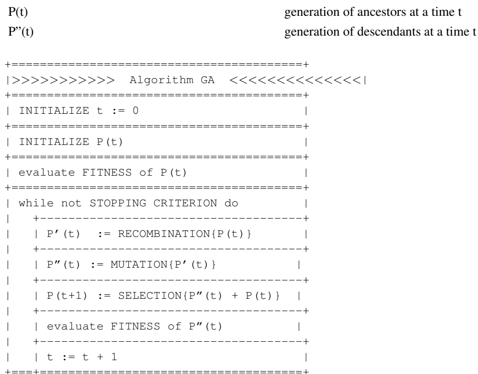
Figure 57-1. Structured Diagram of a Genetic Algorithm
