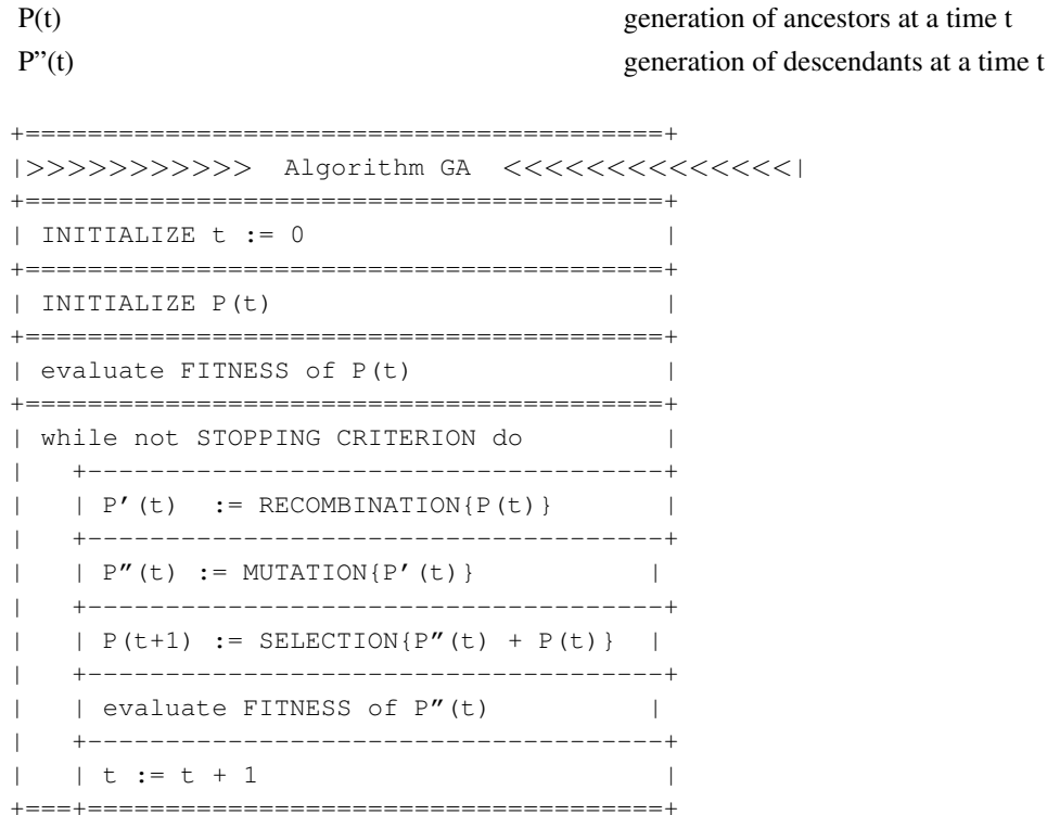
Figure 58-1. Structured Diagram of a Genetic Algorithm
